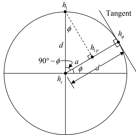
Figure 11: Projecting h_1 along a line parallel to the tangent (as in Figure 7).
