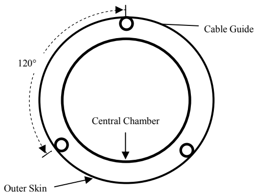
Figure 4: Cross-sectional schematic of the skin and tendon configuration.
