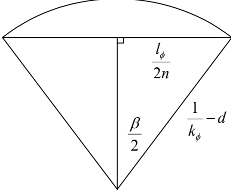
Figure 12: Triangle used to determining cable length l_\phi . (from Figure 9).
